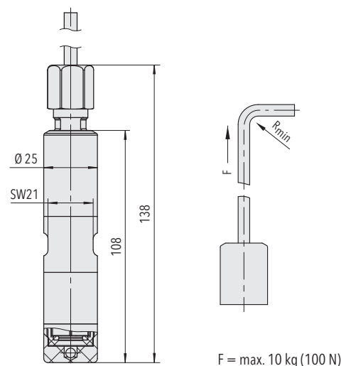
Serto adapter SO 50021-12 for stainless steel tubes with: outer diameter 12 mm inner diameter 8 mm
