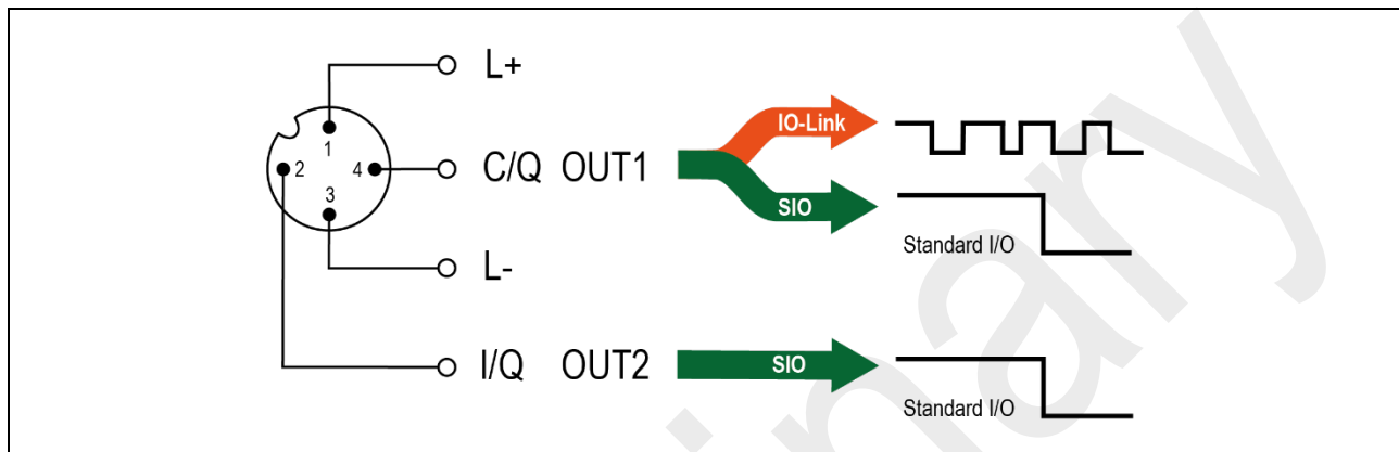
Figure 1 Electrical connection and operating modes
