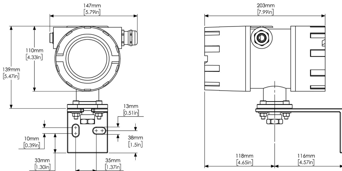
Fig. 3: Dimensional Drawing: TCE 8000 Wallmount
