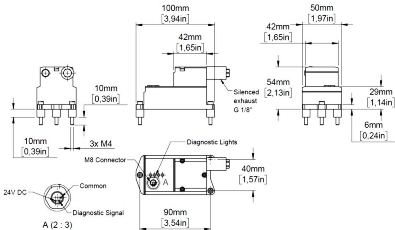
Fig. 4: Dimensional Drawing: Pneumatic Power Generator
