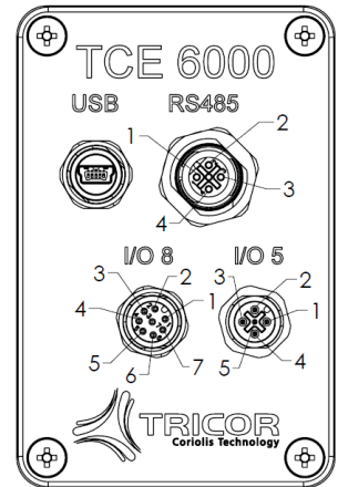
Fig. 6: TCE6000 PIN Assignments
