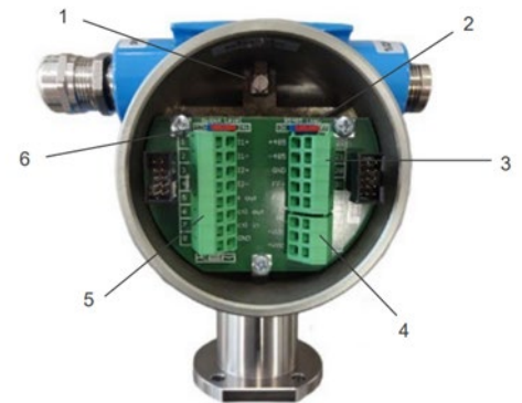
Fig. 7: TCE8000 PIN Assignments
