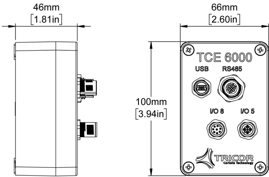
Fig. 1: Dimensional Drawing: TCE 6000
